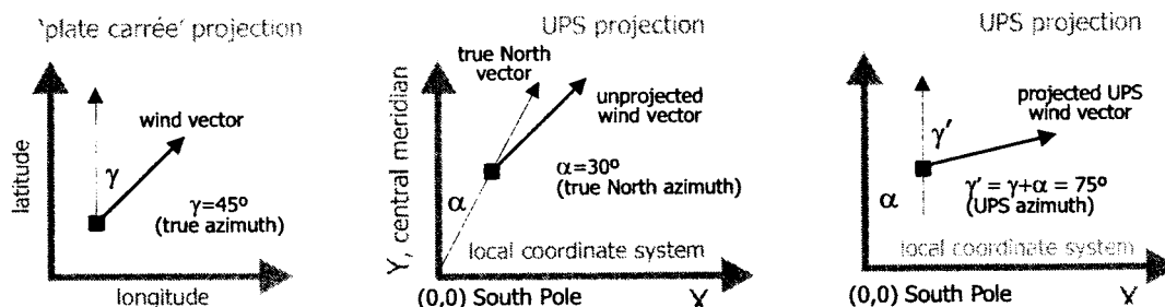
Figure 6. Calculation of azimuth vector in UPS projection.
